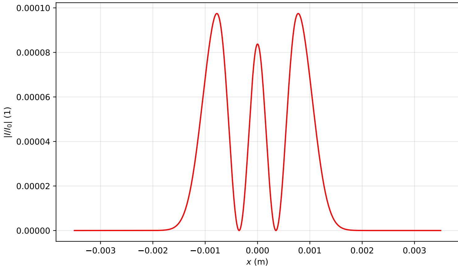
Intensity profile I(x, y = 0, z = 0.239)/I_0 , P_{in}=4.0P_{cr} , artificial time
